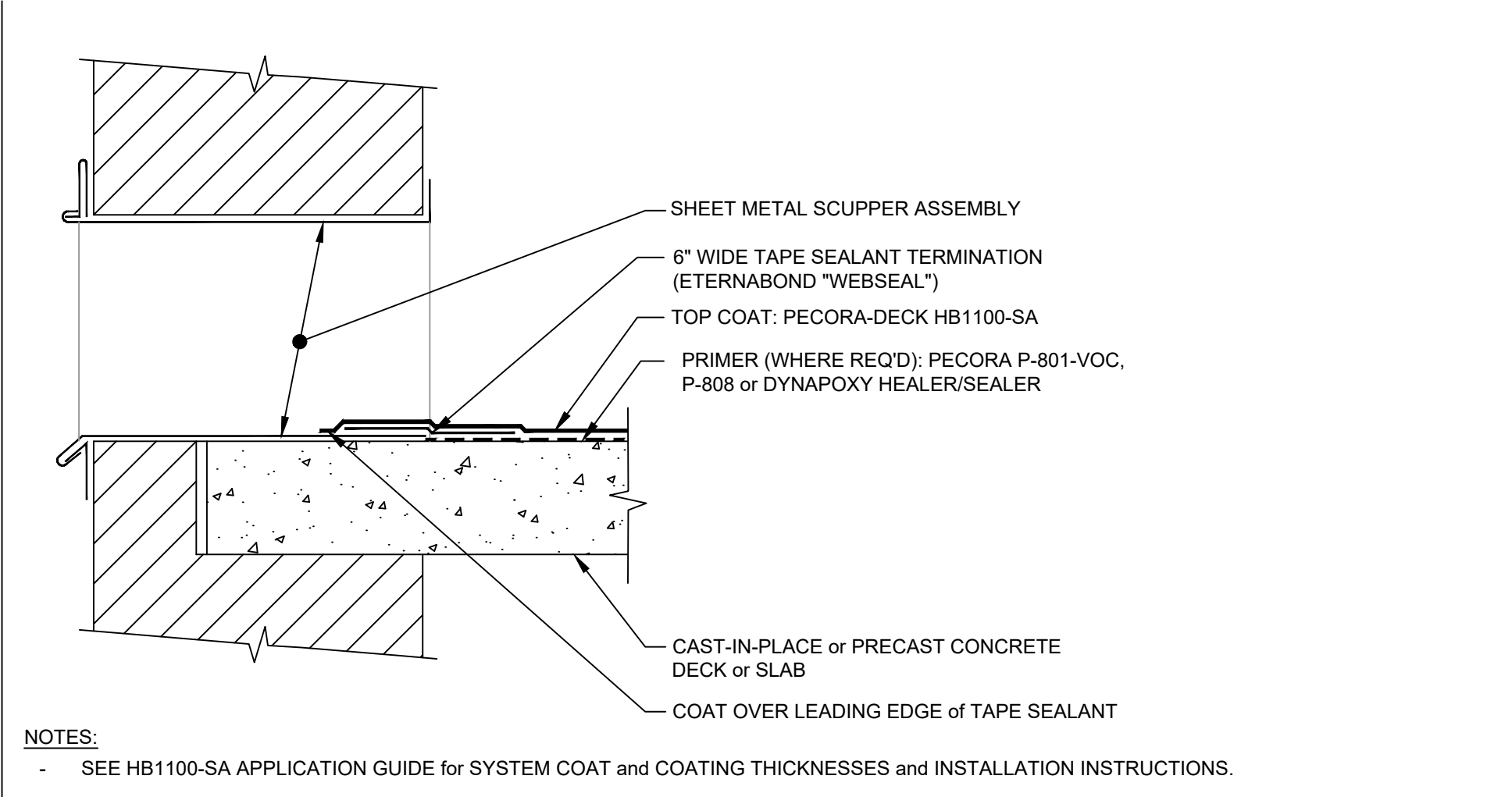
124: SCUPPER DETAIL
