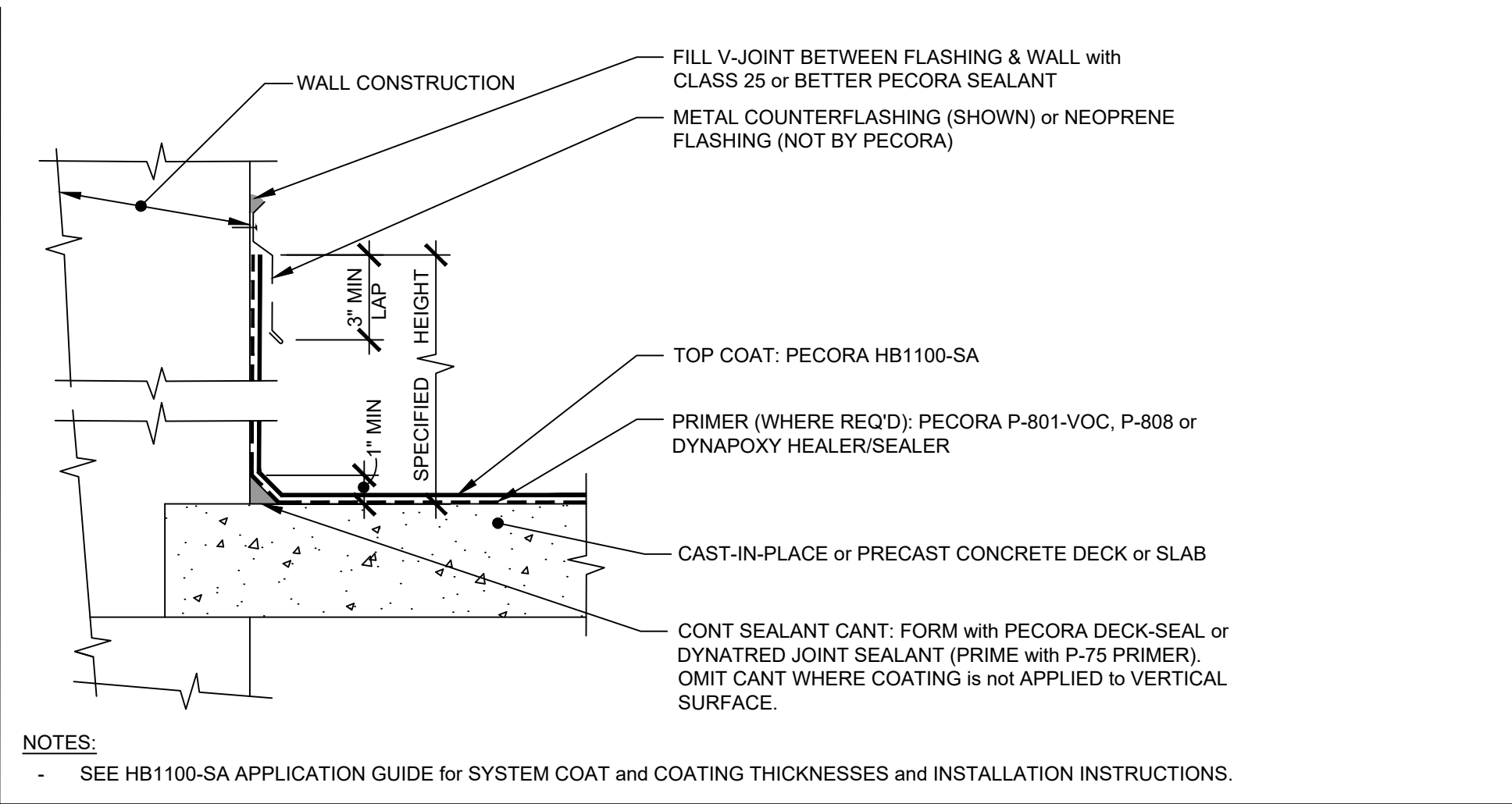
117: DECK-TO-WALL STATIC JOINT
