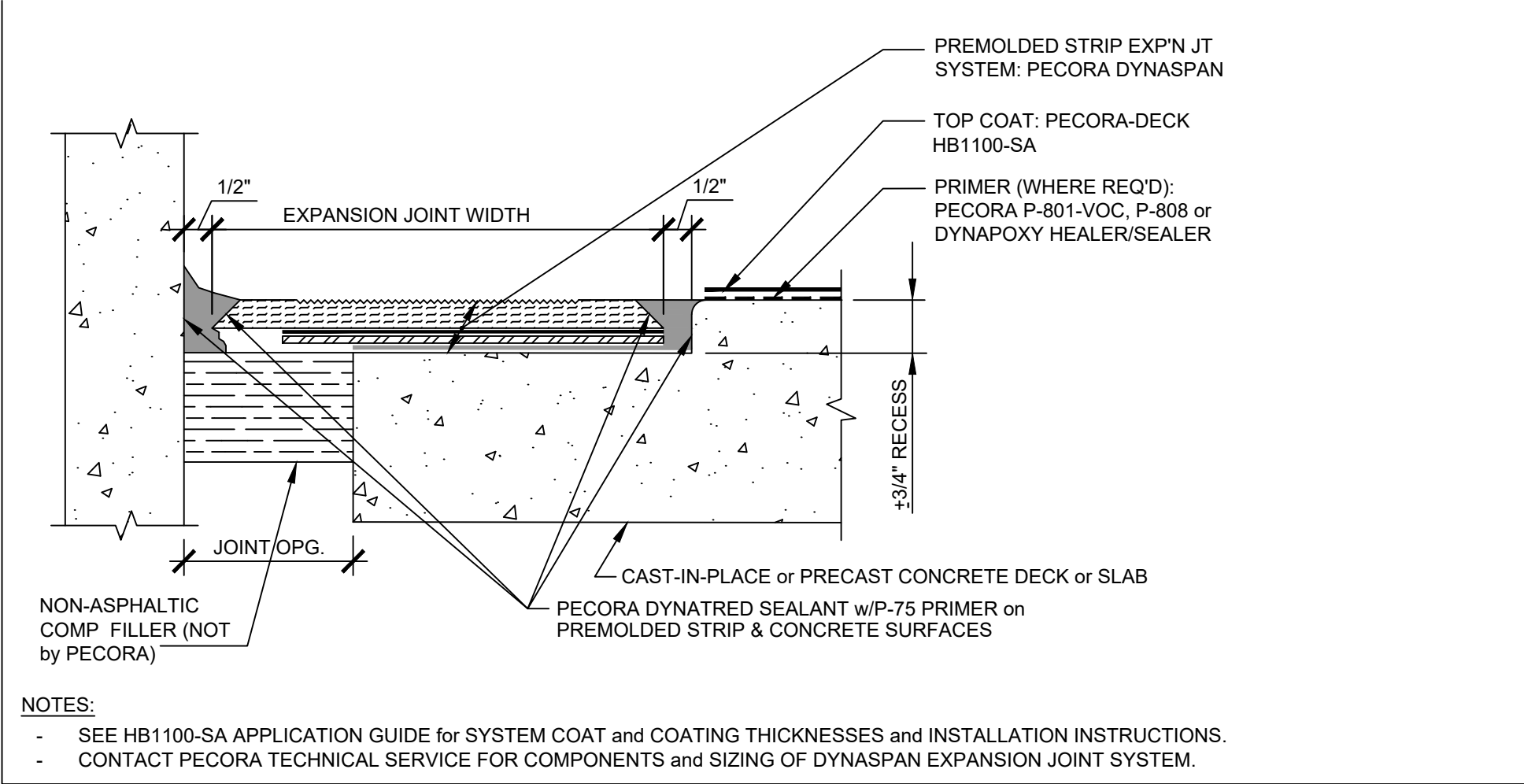
114: DECK-TO-WALL EXPANSION JOINT with PECORA DYNASPAN
