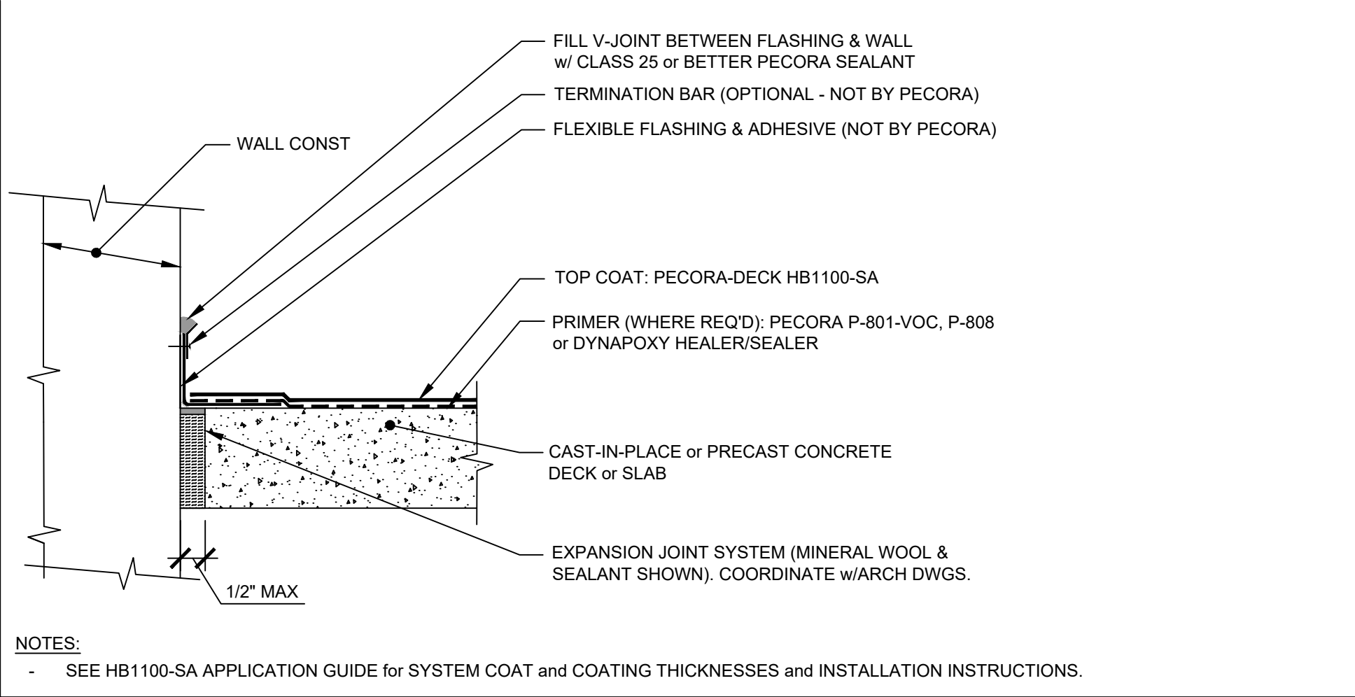
115: DECK-TO-WALL EXPANSION JOINT (FLEXIBLE FLASHING)
