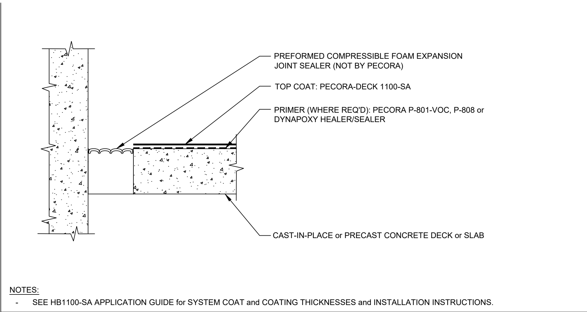
116: DECK-TO-WALL EXP. JT. (COMPRESSIBLE JT FILLER)
